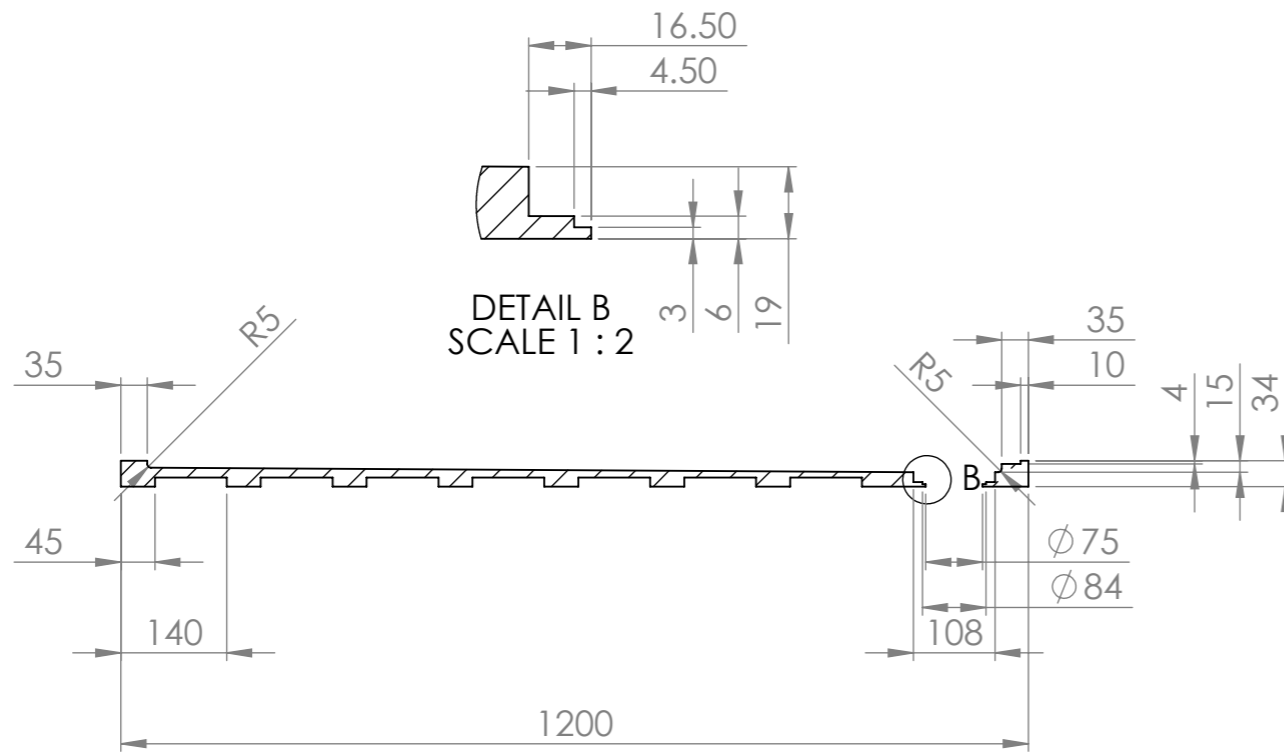
SECTION A-A CROSS SECTION VIEW
